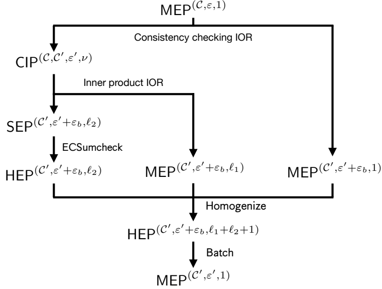
Figure 1: Structure of the CodeSwitch IOR from \text{MEP}^{(\mathcal{C}, \varepsilon, 1)} to \text{MEP}^{(\mathcal{C}', \varepsilon', 1)} where \mathcal{C} is a tensor code. The steps labelled “consistency checking IOR” and “inner product IOR” only apply to the CodeSwitch IOR for tensor codes, but the subsequent reductions are generic and independent of \mathcal{C} .
