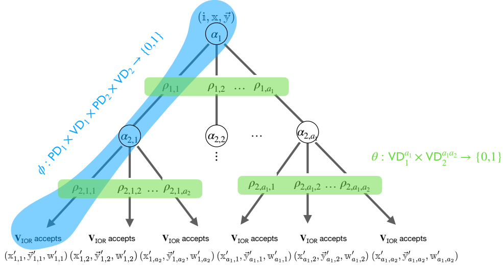
Figure 2: An ((a_1, a_2), \phi, \theta, \mathfrak{i}, \mathfrak{x}, \vec{y}) -constrained transcript tree for an IOR from \mathcal{R} to \mathcal{R}' . Each path from root to leaf ends in \mathbf{V}_{\text{IOR}} accepting, and furthermore must satisfy the vertical predicate \phi . In addition, each label on each leaf is labeled with (\mathfrak{i}', \mathfrak{x}'_{i,j}, \mathfrak{y}'_{i,j}, \mathfrak{w}'_{i,j}) \in \tilde{\mathcal{R}}' , which is the index-instance-witness triple outputted at the end of the IOR interaction. Finally, the verifier challenges on the edges of the tree must satisfy the ‘challenge predicate’ \theta: \text{VD}_1^{a_1} \times \text{VD}_2^{a_1 a_2} \rightarrow \{0,1\} . We depict one application of the vertical predicate \phi (blue) and the application of the challenge predicate \theta (green) in the figure.
