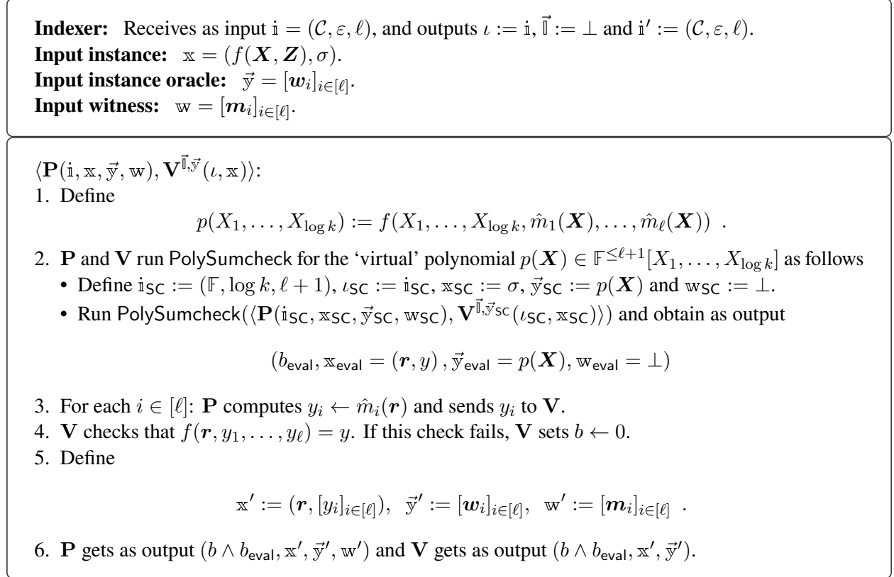
Figure 4: ECHsumcheck, an IOR from \text{SEP}^{(\mathcal{C}, \varepsilon, \ell)} to \text{HEP}^{(\mathcal{C}, \varepsilon, \ell)}
