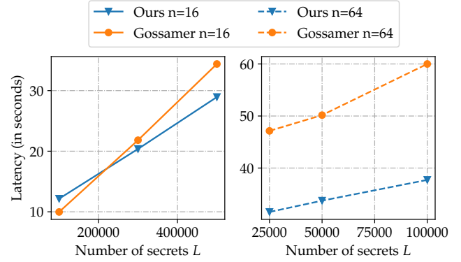
Figure 3: Our protocol vs Gossamer: Latency of our linear cost DPSS protocol vs Gossamer in a geo-distributed testbed with n = 16, 64 parties. At n = 16 , our work scales better than Gossamer beyond L = 300000 secrets, whereas at n = 64 , our protocol is better at all L .
