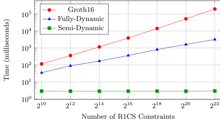
Fig. 4: Update time (serial) of DYNARK with d = 1 .
