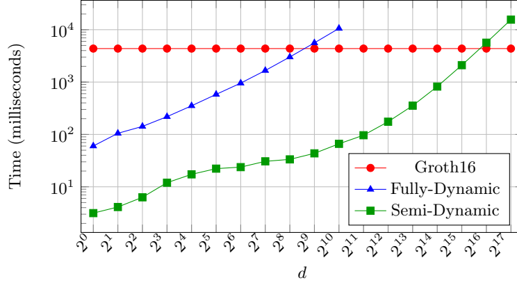
Fig. 3: Update time (parallel) of DYNARK with different d and n = 2^{20} .
