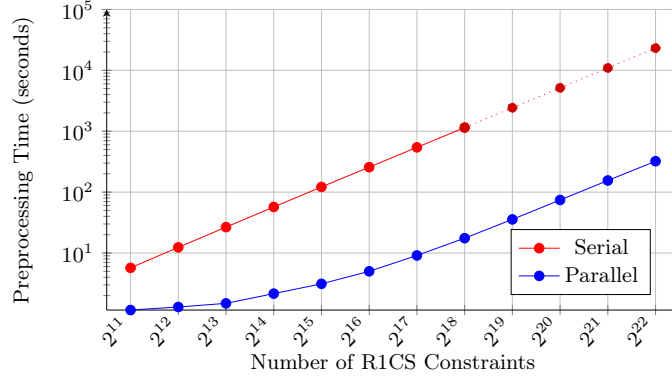
Fig. 1: Preprocessing Time
