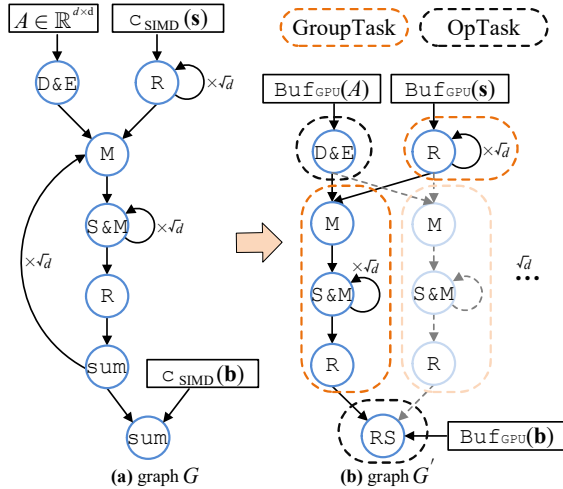
Figure 6: Operation flow graph for computing A \cdot s + b in the gpu IR. D&E denotes diagonal extraction and plaintext encoding, R refers to Rotate, M depicts plaintext-ciphertext multiplication, S&M indicates accumulation after plaintext-ciphertext multiplication, sum specify ciphertext addition, and RS is the reduce-sum operator.
