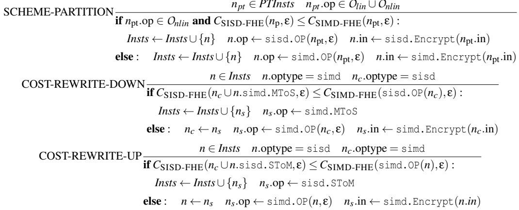
Figure 5: Cost-based cross-scheme graph rewriting rules in Libra. PTInsts represents plaintext nodes, O is linear or nonlinear operator set, Insts represents ciphertext nodes, C_{Scheme} denotes a node’s computational cost under the current scheme, and \epsilon denotes its precision constraint.
