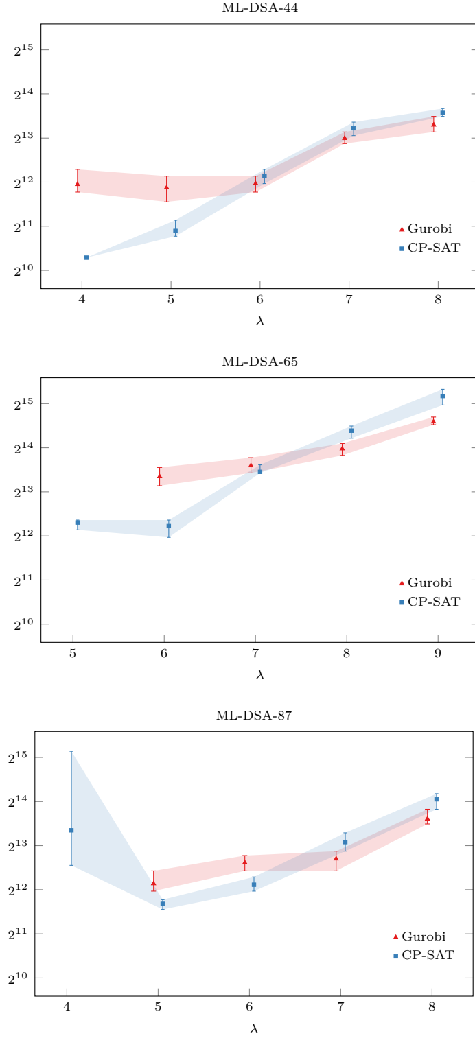
Figure 6: Number of informative signatures with exact leakage required for key recovery via solving ILP 1 using Gurobi’s feasibility pump (4 cores) and CP-SAT (64 cores), each with a 10-minute time limit per experiment: minimum, maximum, and average value across 10 experiments per data point.
