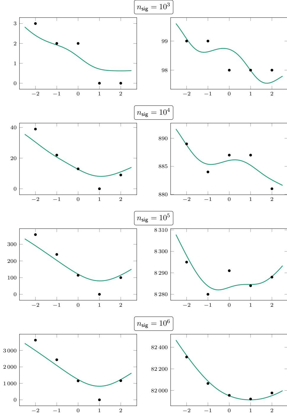
Figure 8: Coordinate slices x_j \mapsto \sum_{i=1}^{n_{\text{sig}}} \psi(t^{(i)}(x)) (dots) and x_j \mapsto \sum_{i=1}^{n_{\text{sig}}} \psi_{\text{approx}}(t^{(i)}(x)) (curves, scaled) with the other coordinates fixed either to the coordinates (x_{j'}^*)_{j' \neq j} of the true key (plots on the left) or to a random vector with entries in [-\eta, \eta] \cap \mathbb{Z} (plots on the right); example for the parameter set ML-DSA-44 with \lambda = 6 , p_{\text{err}} = 0 , and x_j^* = 1 .
