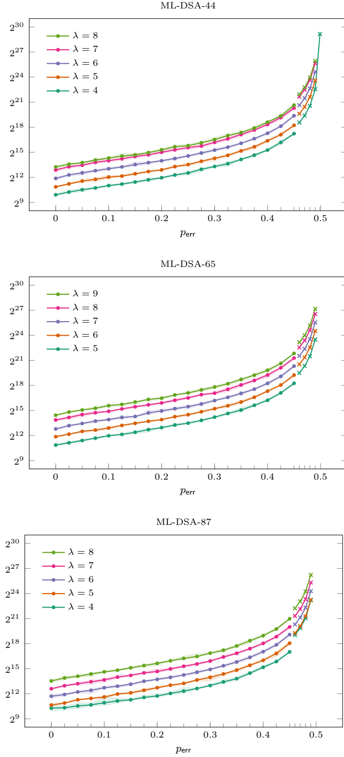
Figure 11: Number of informative signatures with noisy leakage required for key recovery using the NLP attack: minimum, maximum, and average value across 10 experiments per data point (dots), and value for which all out of 10 experiments succeeded (crosses).
