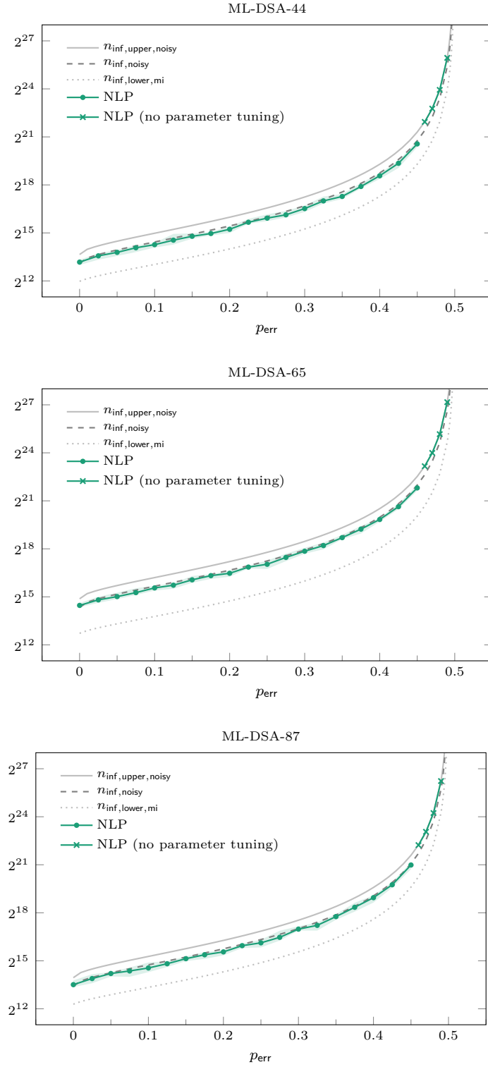
Figure 5: Estimates in the high- \lambda regime for the expected number of signatures required for key recovery, together with experimental results from Figure 11 for comparison.
