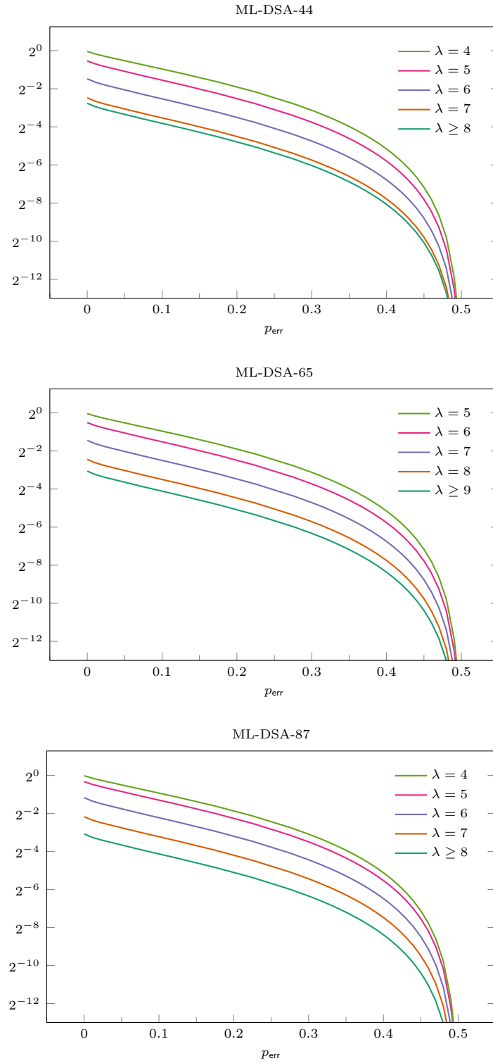
Figure 3: Bits of information I(X^*; C_{\text{inf}}, Z_{\text{inf}}, \tilde{Y}_{\lambda, \text{inf}}) contained on average in an informative leaky signature about the key.
