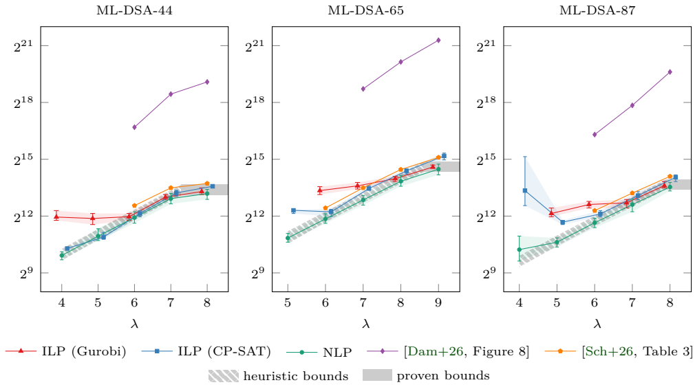
Figure 1: Summary of results for exact leakage; number of informative signatures needed.
