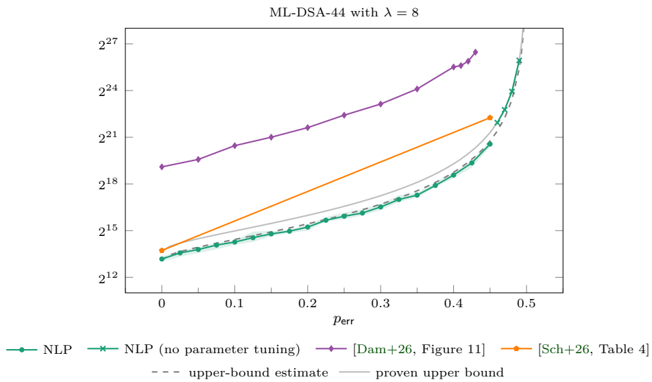
Figure 2: Summary of results for noisy leakage; number of informative signatures needed.
