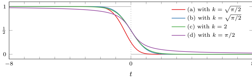
Figure 7: Examples for continuous approximations \psi_{\text{approx}} of \psi on [-2^{\lambda-1}, 2^{\lambda-1}] .
