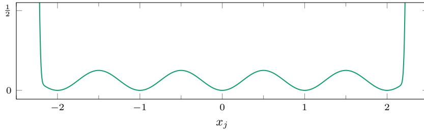
Figure 9: Coordinate slices \psi_{\text{penalty}}(0, \dots, x_j, \dots, 0) in the situation \eta = 2 with parameter values w_{\text{int}} = \frac{1}{5} , w_{\text{box}} = 5 , \eta_+ = \eta + \frac{1}{4} , k = 40 .
