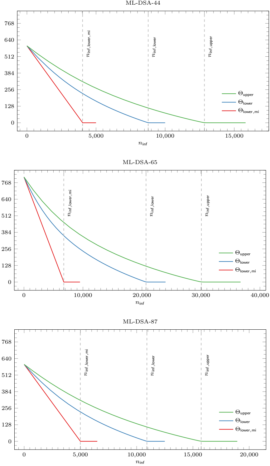
Figure 4: Binary logarithm of the lower and upper bounds for \mathbb{E}(\#\mathcal{X}_{\text{cand},\text{inf}}) .
