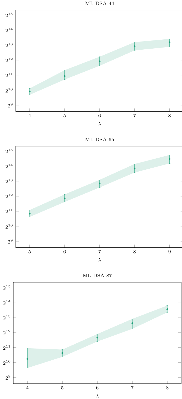
Figure 10: Number of informative signatures with exact leakage required for key recovery using the NLP attack: minimum, maximum, and average value across 100 experiments.
