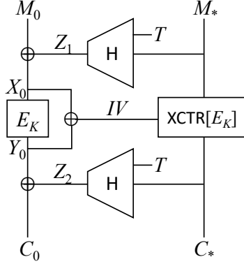
Fig. 1. HCTR2. The hash key is defined as E_K(0) and the mask value of XCTR L = E_K(1) is included in XCTR.
