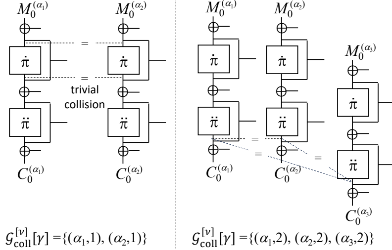
Fig. 5. Collision sets with a single collision (left) and with a 3-multi-collision (right) where the right parts of CHCTR2 are omitted.
