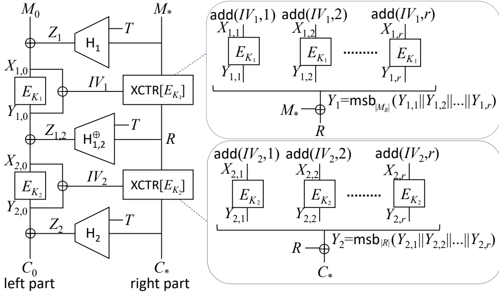
Fig. 4. CHCTR2. r = |M_*|_n . H_1 := H_{H_1} and H_2 := H_{H_2} . The hash keys are defined as H_1 = E_{K_1}(\text{bin}_n(0)) and H_2 = E_{K_2}(\text{bin}_n(0)) . The second hash value is defined as Z_{1,2} = H_{1,2}^\oplus(T, R) = H_1(T, R) \oplus H_2(T, R) .
