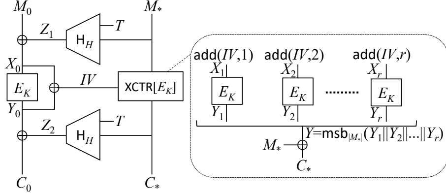
Fig. 3. HCTR2 and XCTR. The hash key is H = E_K(\text{bin}_n(0)) . r = |M_*|_n .
