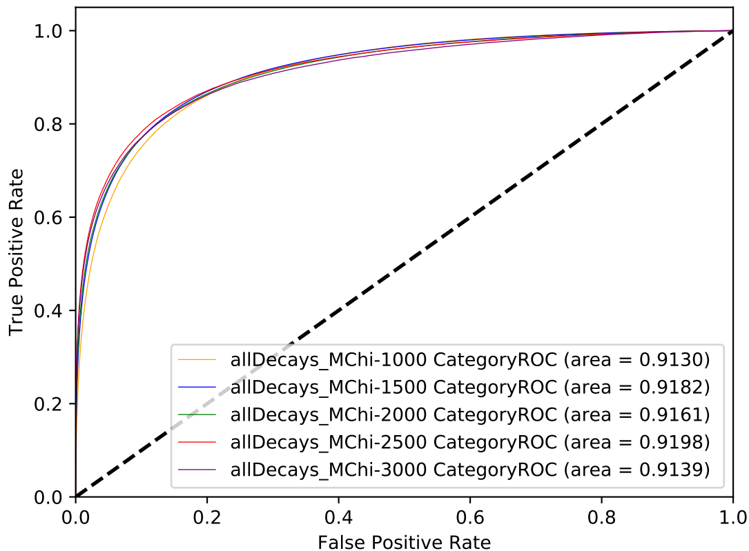
combine ROC Curve
