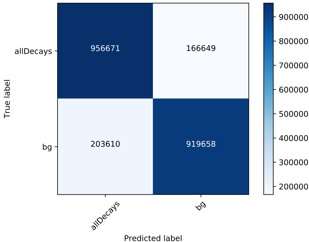
combine Confusion Matrix
