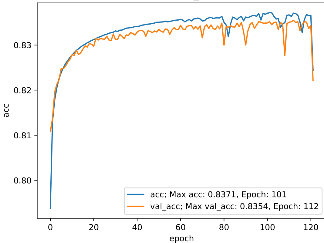
combine acc and val_acc vs. epochs
