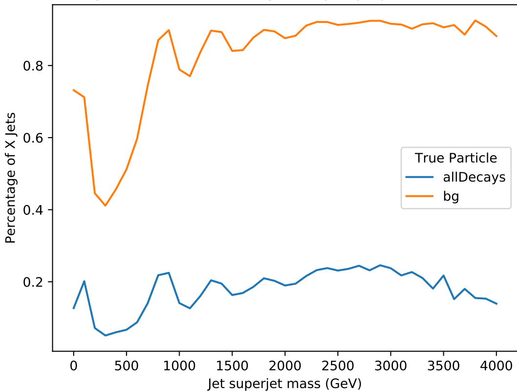
Percentage of X Classified as bg Jets by superjet mass for combine
