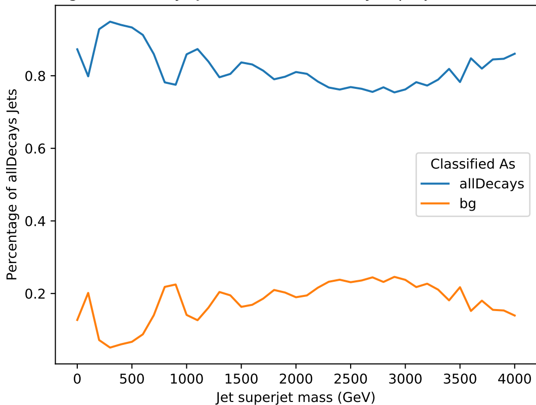
Percentage of allDecays Jets Classified as X by superjet mass for combine
