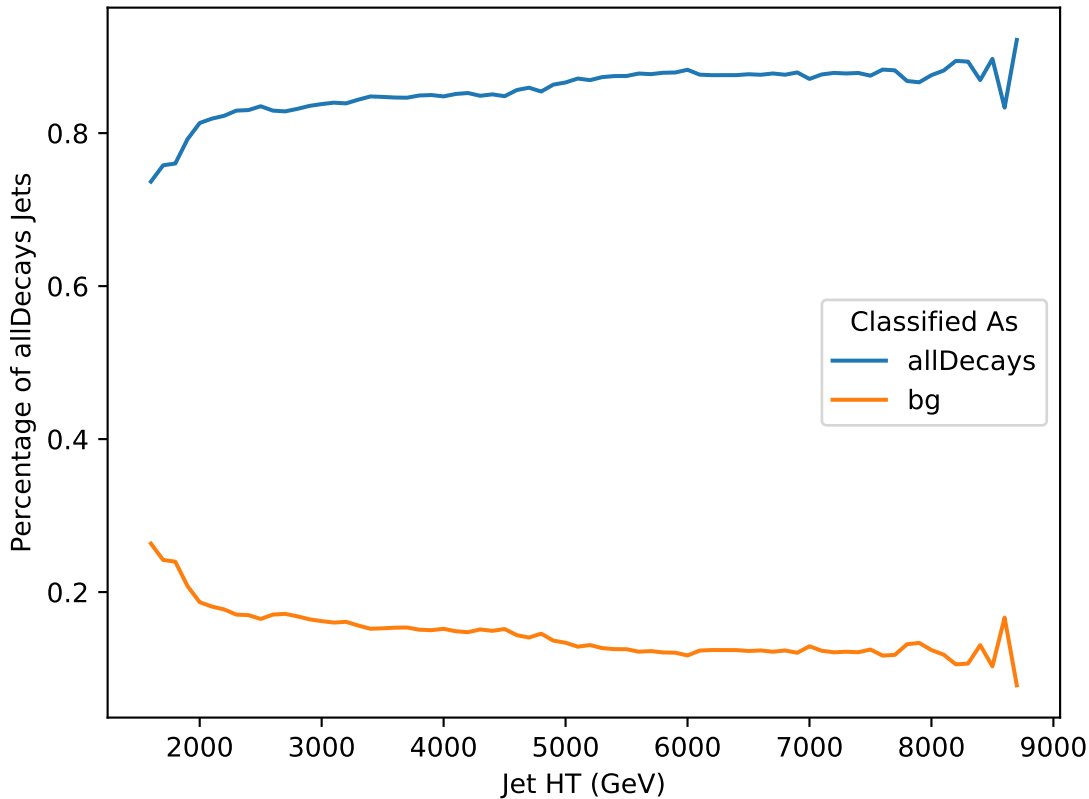
Percentage of allDecays Jets Classified as X by HT for combine
