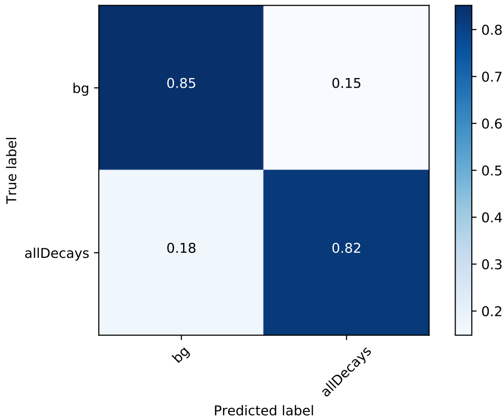
combine Normalized Confusion Matrix
