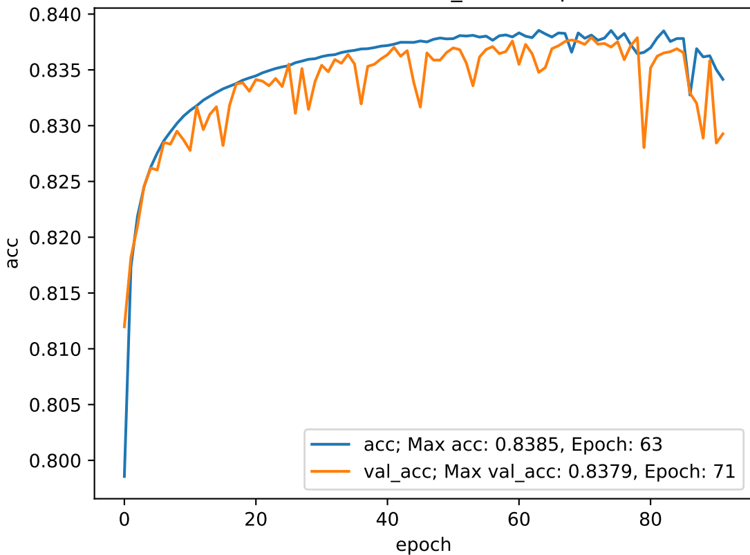
combine acc and val_acc vs. epochs
