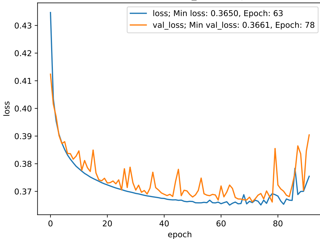
combine loss and val_loss vs. epochs
