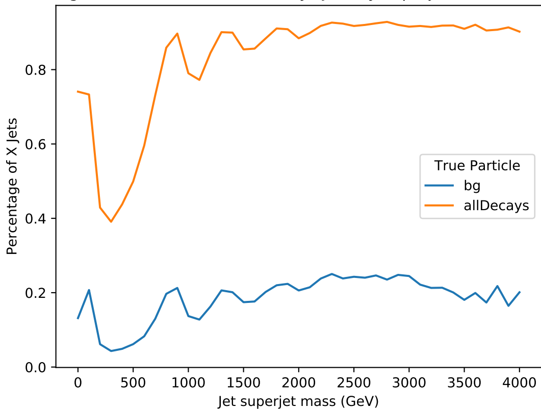
Percentage of X Classified as allDecays Jets by superjet mass for combine
