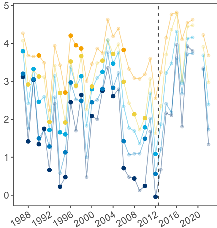
Bottom temperature
