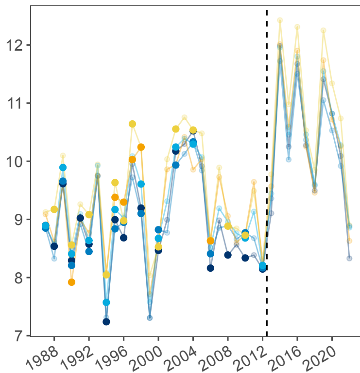
Surface temperature
