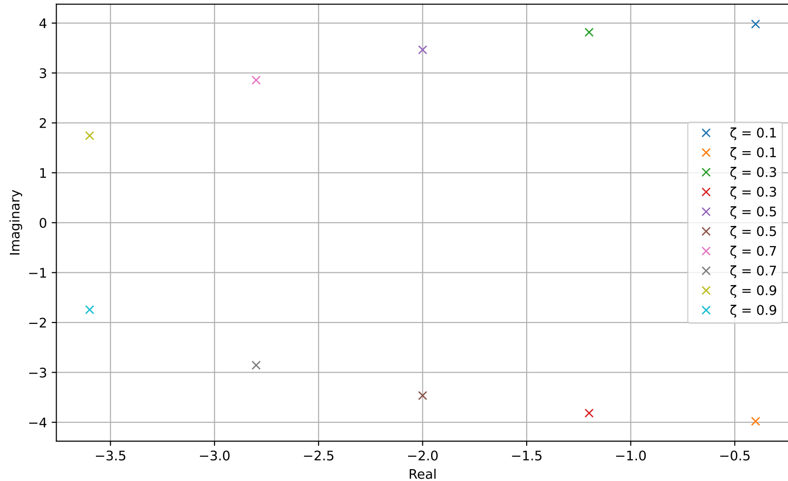
Poles of MSD System
