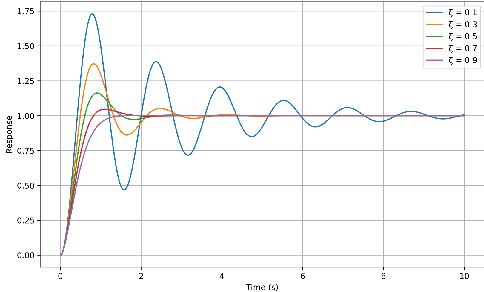
Step Response of MSD System
