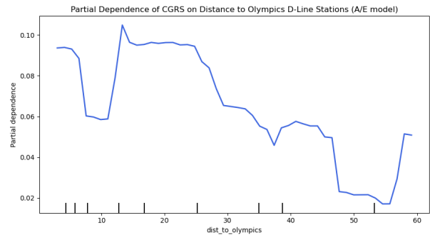
(b) dist_to_olympics
