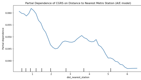
(a) dist_nearest_station
