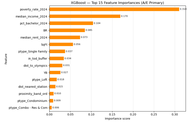
(b) XGBoost
