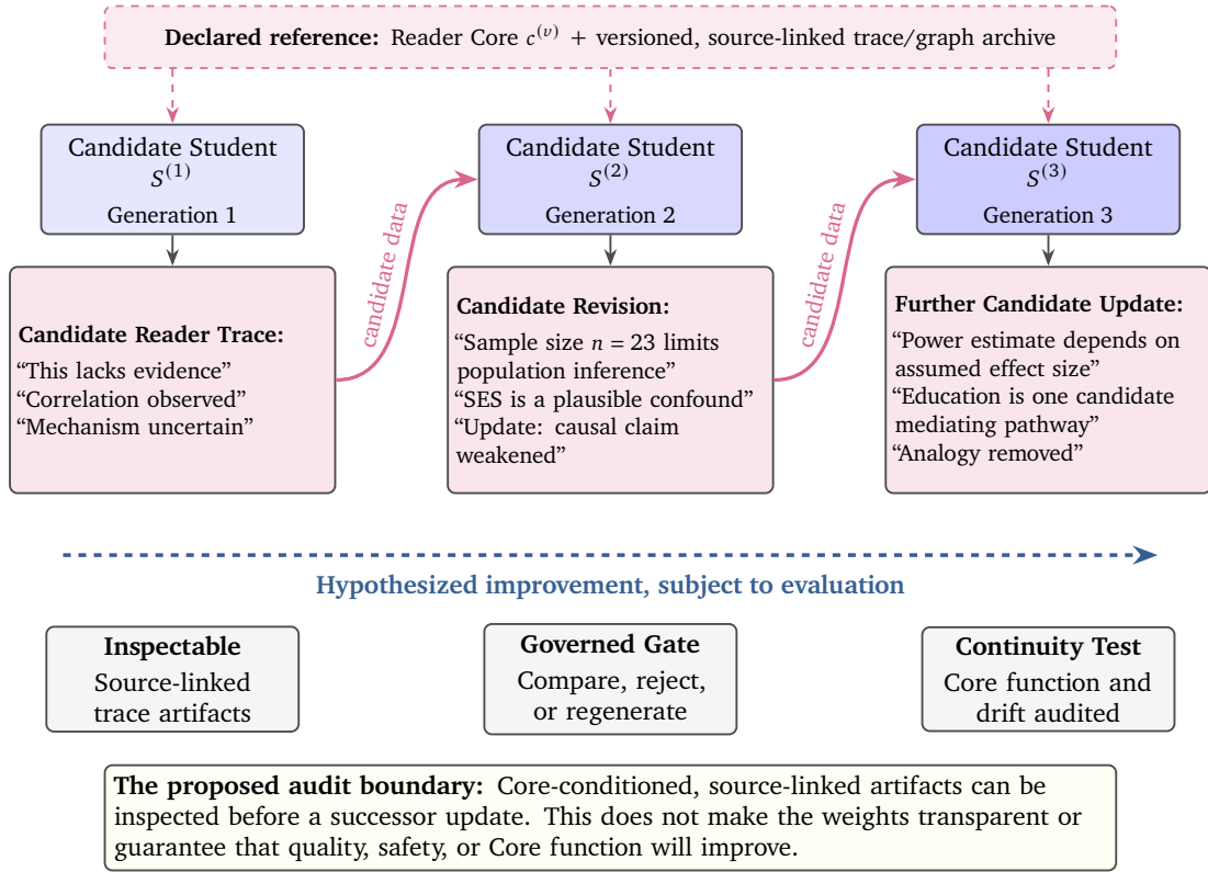
Figure 3: The Reader-Anchored Successor-Training Loop. Candidate improvement is routed through source-linked trace artifacts that can be inspected before compression into successor weights; the interface is partial and does not make the resulting Student transparent or safe by itself.
