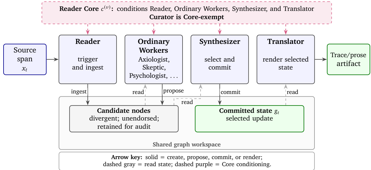
Figure 4: One Teacher-side annotation step of the Metabolic Cycle. In the reference implementation, the Reader, ordinary Workers, Synthesizer, and Translator are Core-conditioned; the Curator is the exception. Workers propose candidate nodes in the shared graph workspace, the Synthesizer selects and commits an update, and the Translator renders the committed state. Core placement and the value of specialized roles remain unrun ablations.
