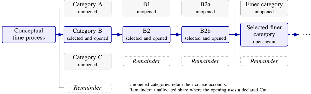
Figure 1: Recursive conceptual decomposition of a process. Finer categories and their relationships explain the selected parent; further openings deepen that explanation. Selecting B, then B2, then B2b exposes finer categories while their siblings remain at their existing resolution. The levels show conceptual depth, not successive periods; the final arrow indicates that opening can continue. Blue marks the selected branch. This is a selected view, not a requirement to construct a complete tree.
