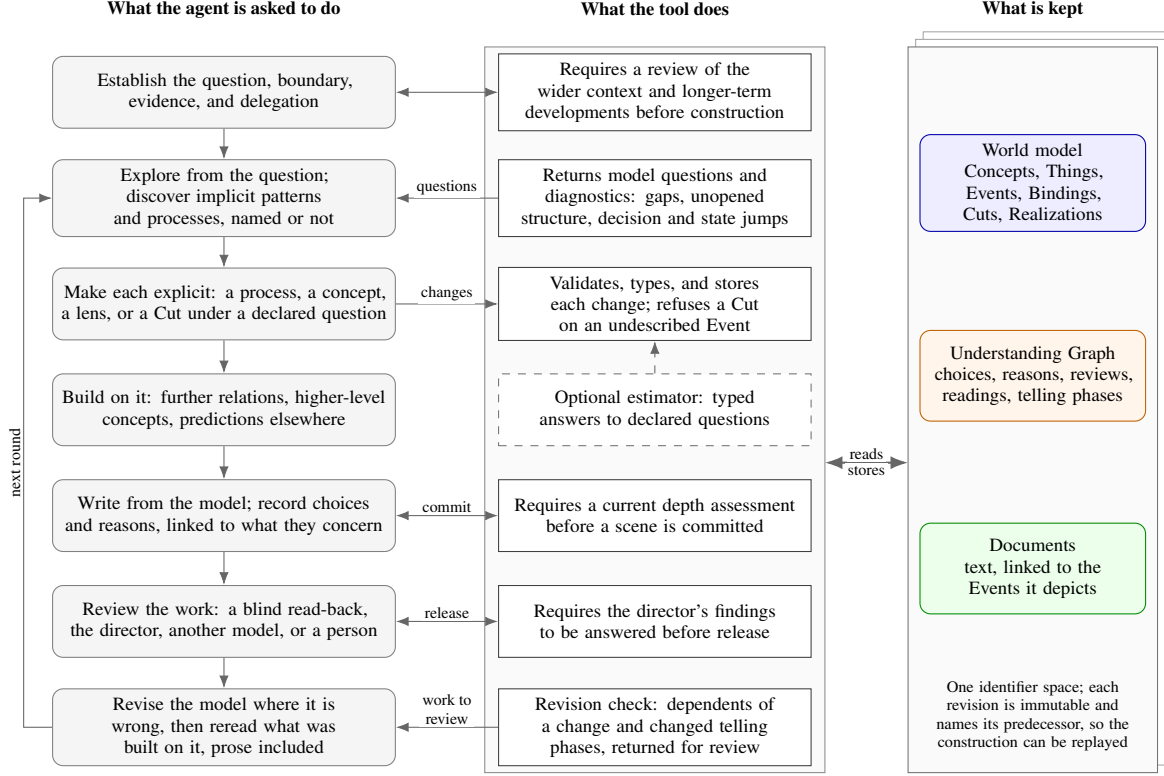
Figure 5: The construction loop. Left: what the shared instructions ask the calling language model to do. The order is a guide rather than a fixed sequence; any step may lead back to exploration, and each round builds on the account the previous one left. Middle: what deterministic tool code does. It validates and stores every change, returns questions after each one, refuses gated operations until the required reviews exist and their findings are answered, and lists the work a revision makes due. The estimator is optional, and the scene and release gates belong to the storytelling add-on. Right: the one versioned record that every step reads and changes through the tool. The tool checks records and their declared links; it does not supply the interpretations or certify that an account is adequate.
