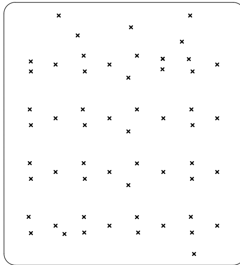
Drill Map: x 0.254mm / 0.0100" (57 holes)
