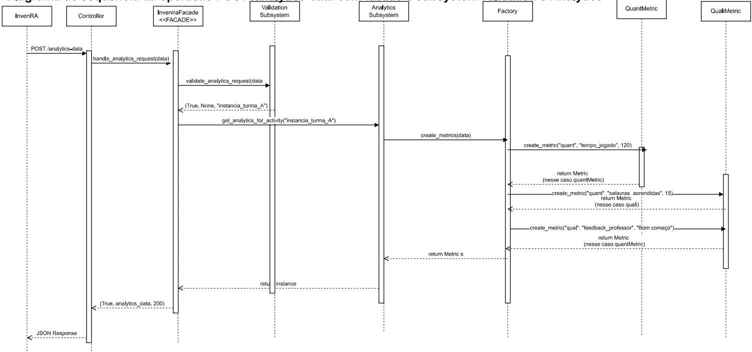
Diagrama de sequencia da operacao POST /analytics-data com facade e subsystem validation e Analytics
