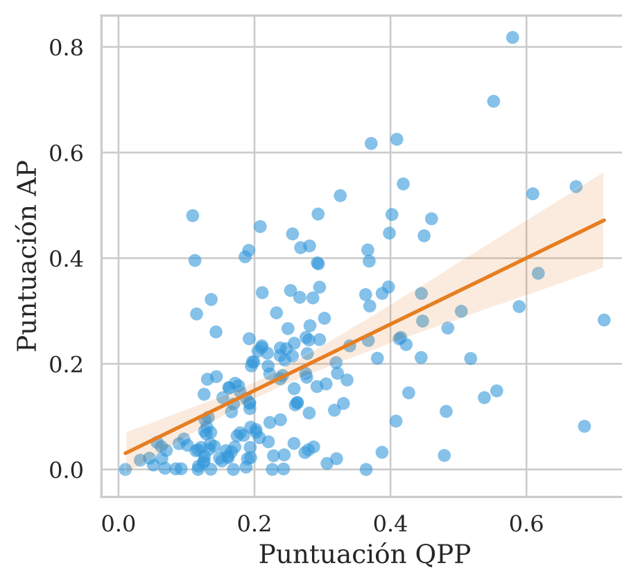
UEF-NQC \tau = 0.4102
