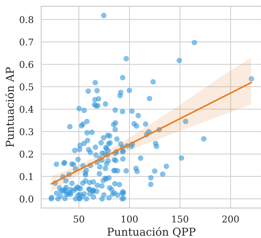
UEF-Clarity \tau = 0.2980
