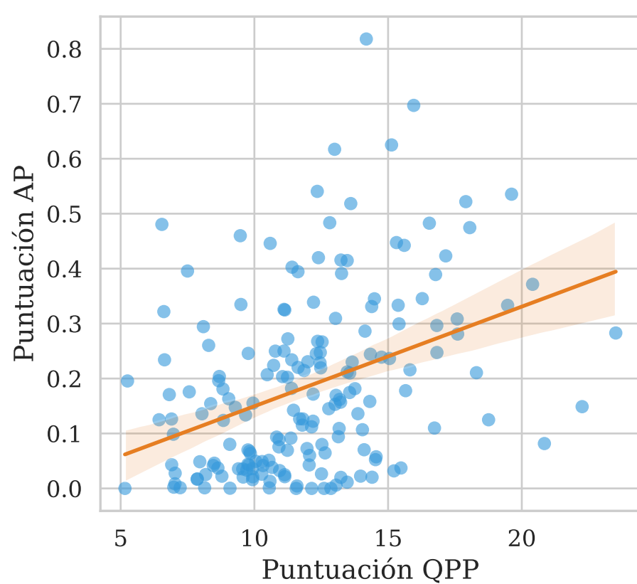
WIG \tau = 0.2685
