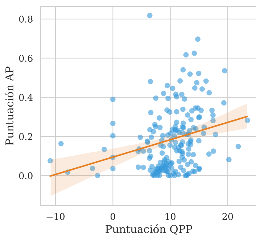
UEF-WIG \tau = 0.2252
