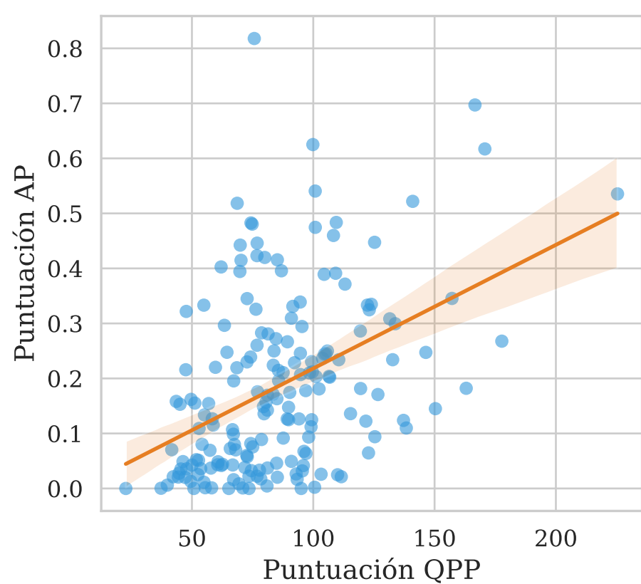
Clarity \tau = 0.2910
