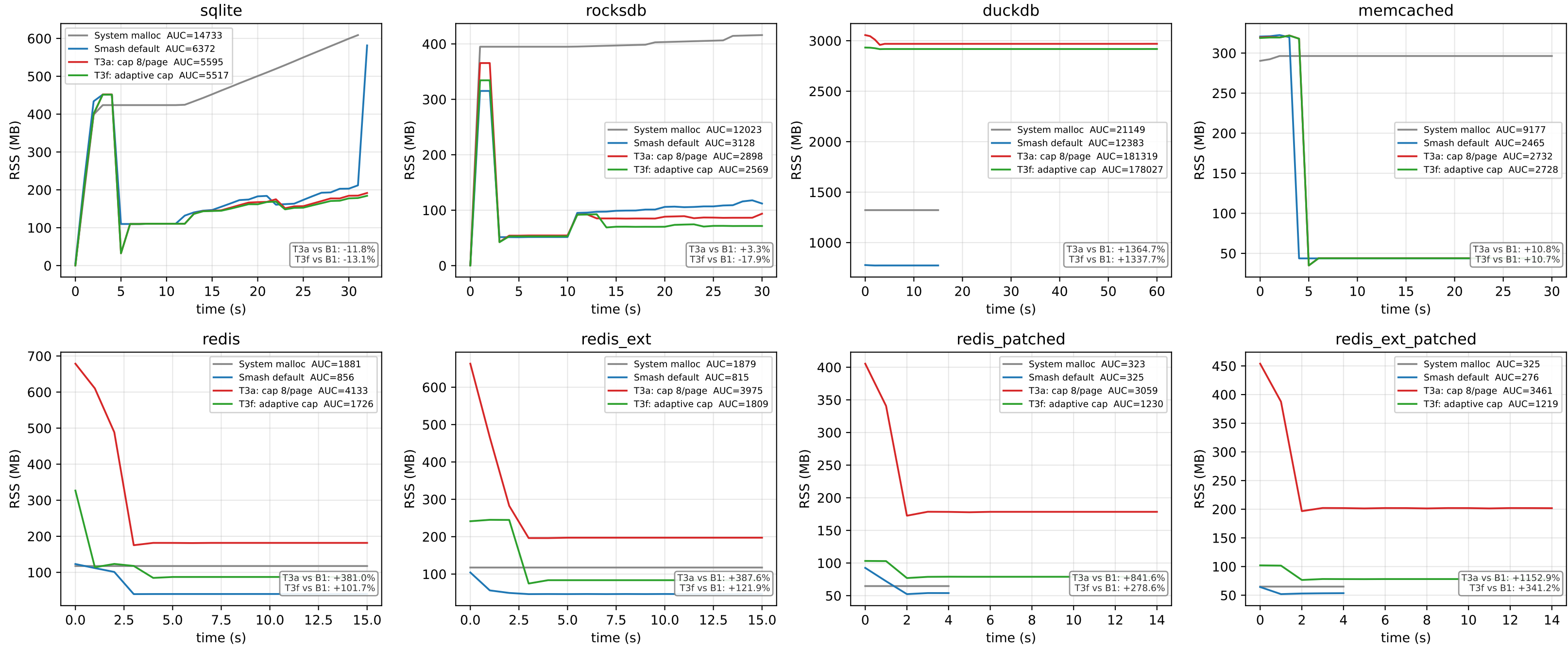
RSS-over-time — AUC for B0 (system) vs B1 (Smash default) vs T3a (unconditional cap) vs T3f (adaptive cap)
