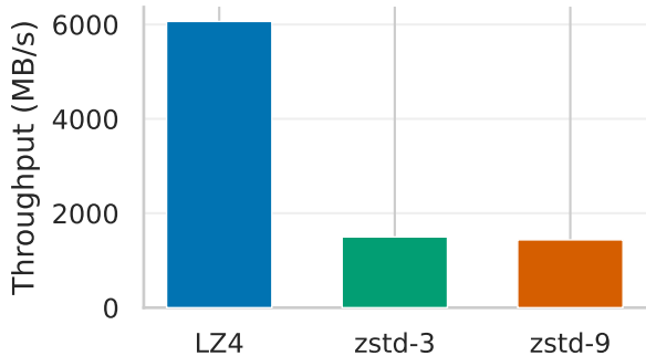
Decompression
