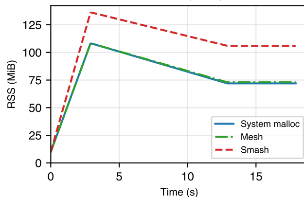
Memcached (macOS)
