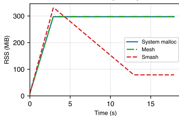
Memcached (macOS)
