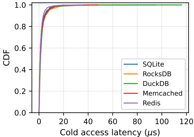
Cold Access Latency CDF
