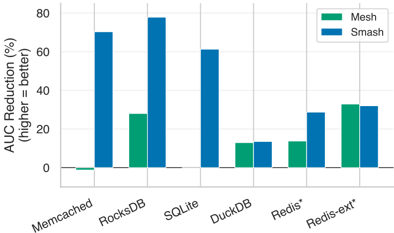
Memory Pressure Over Time (AUC)
