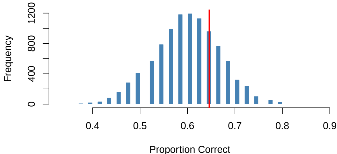
Null Distribution — Proportion Correct
