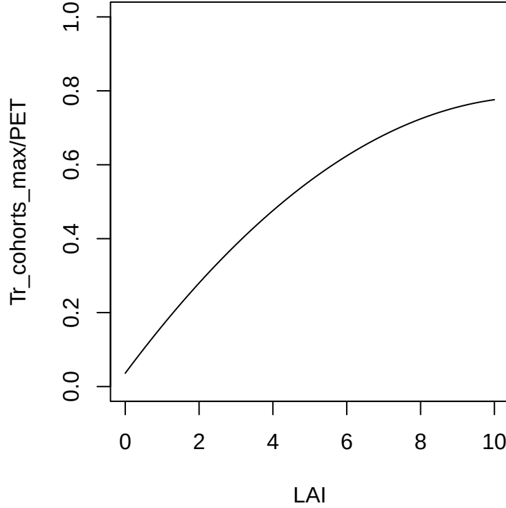
Figure 6.1: Empirical relationship between Tr_{cohorts,max}/PET and LAI_{act}
