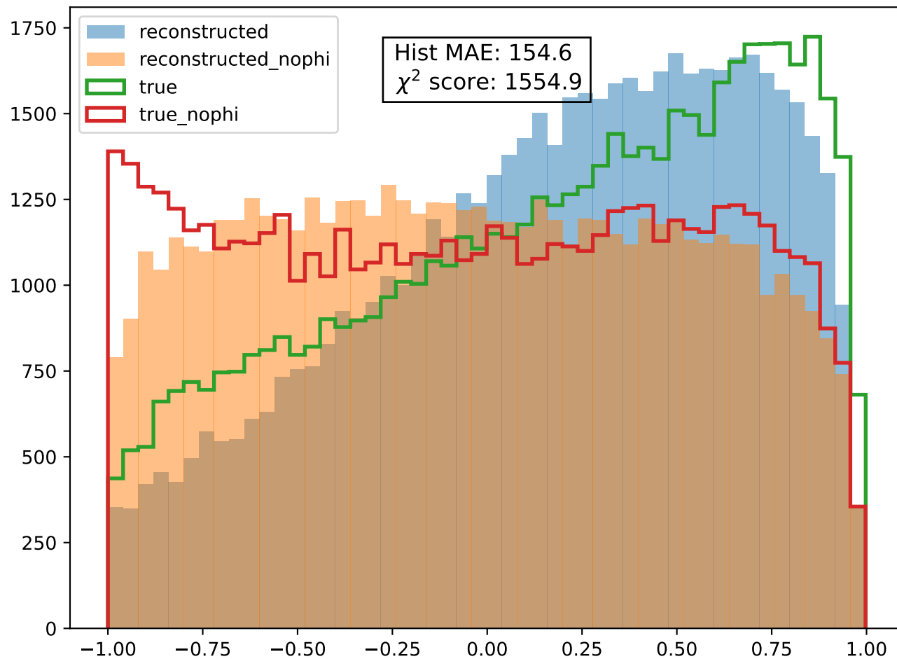
\cos(\mu, d)_{TRF} reconstruction, DM, DELPHES level, MLP
