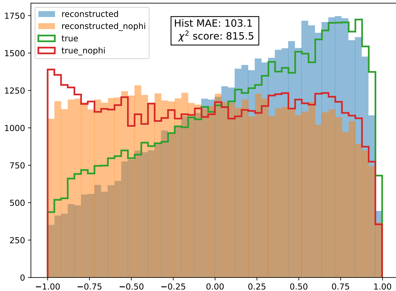
\cos(\mu, d)_{TRF} reconstruction, DM, DELPHES level, \nu -Flows
