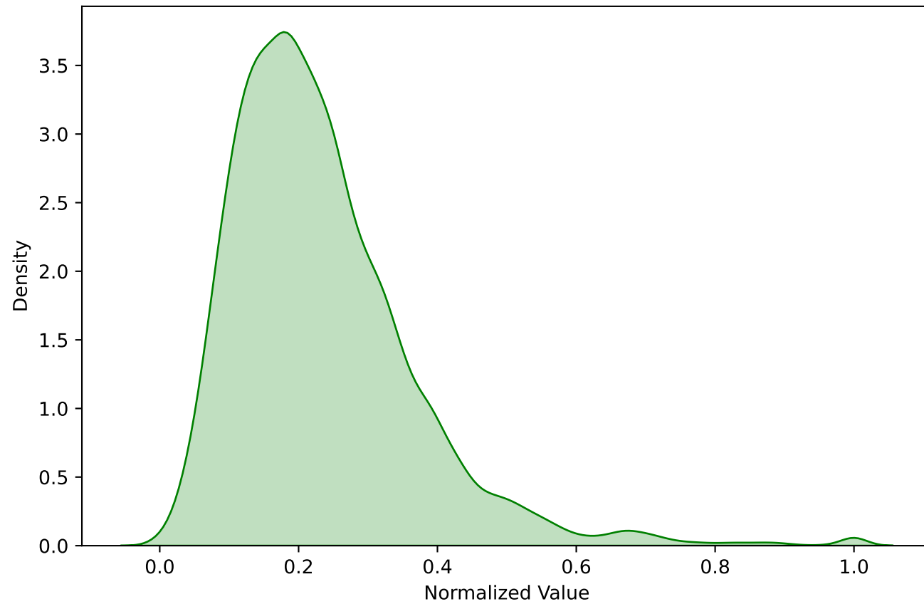
MinMaxScaler (Bounded [0, 1])
