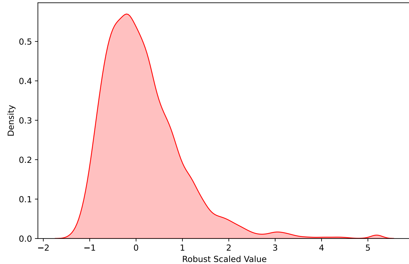
RobustScaler (IQR-Based)
