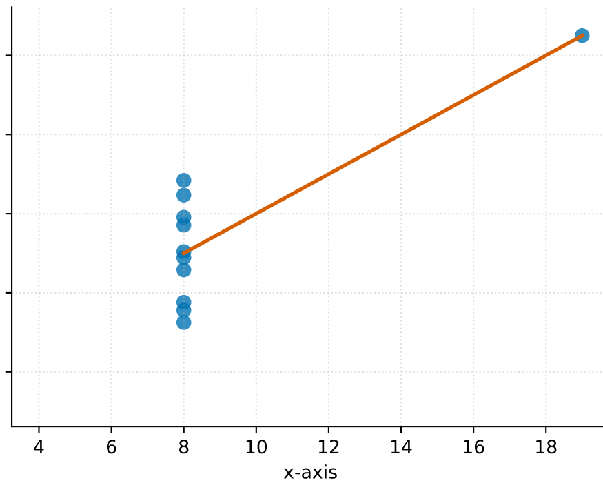
Panel IV ( \bar{x}=9.0 , \bar{y}=7.50 , \text{Var}(x)=11.0 )
