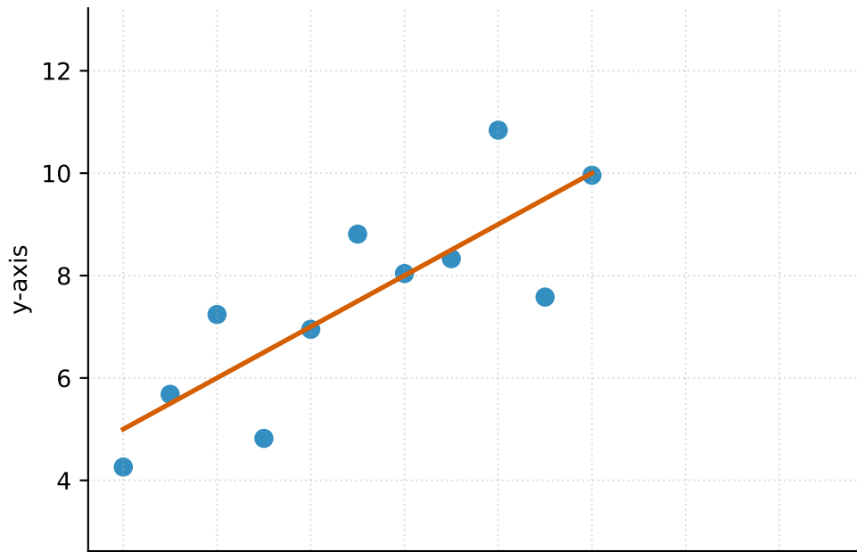
Panel I ( \bar{x}=9.0 , \bar{y}=7.50 , \text{Var}(x)=11.0 )
