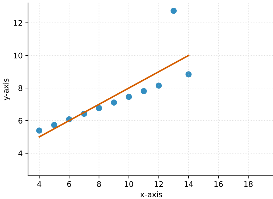
Panel III ( \bar{x}=9.0 , \bar{y}=7.50 , \text{Var}(x)=11.0 )
