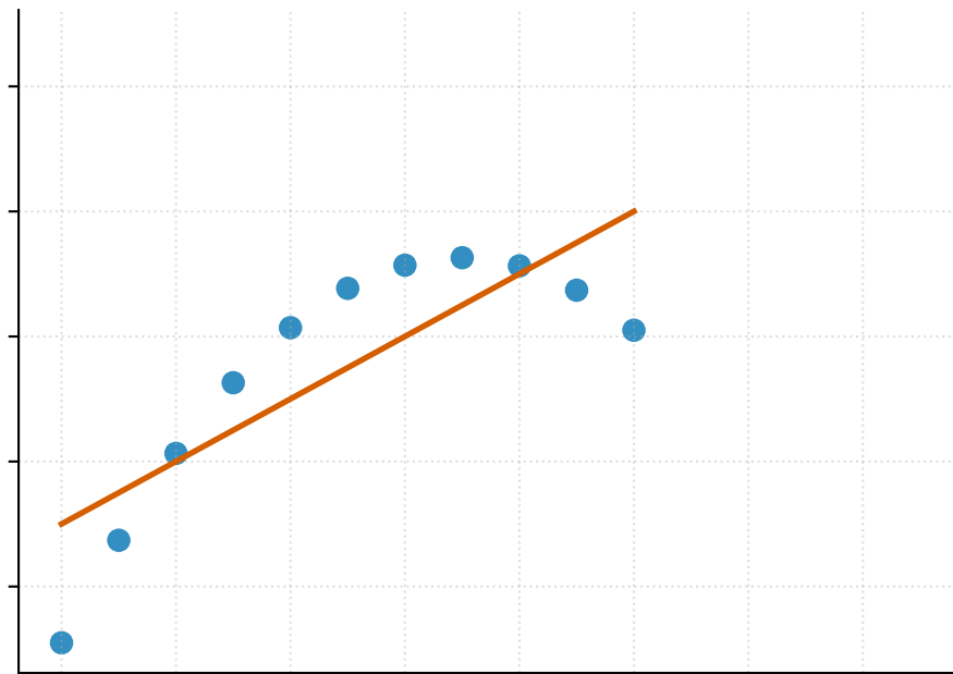
Panel II ( \bar{x}=9.0 , \bar{y}=7.50 , \text{Var}(x)=11.0 )
