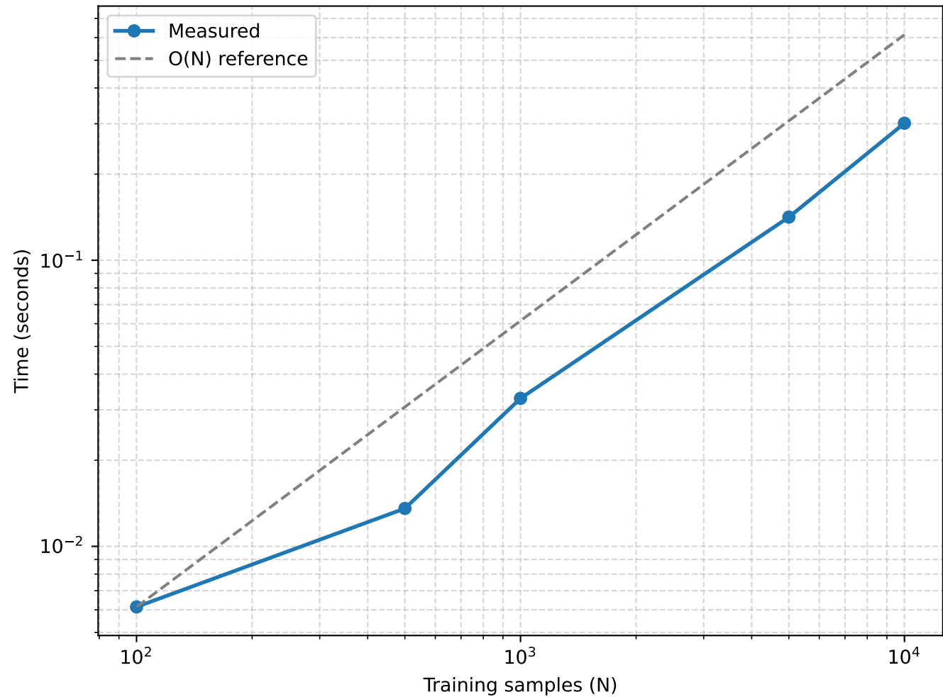
KNN Prediction Time vs Training Size (M=100)
