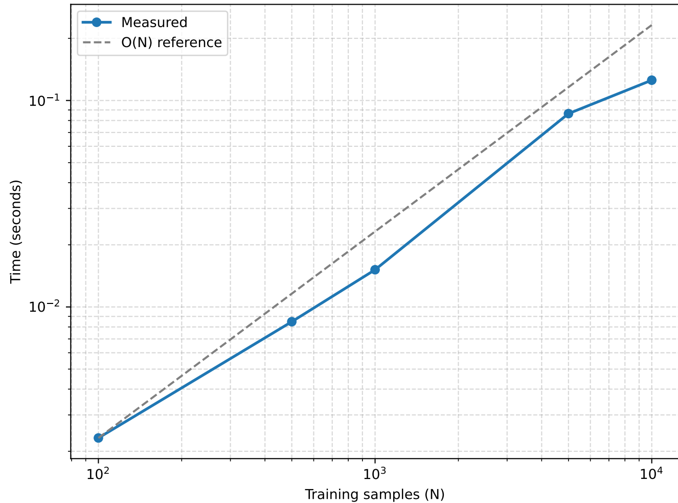
KNN Prediction Time vs Training Size (M=100)
