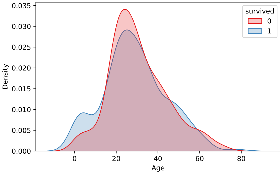
Age Distribution by Survival Status
