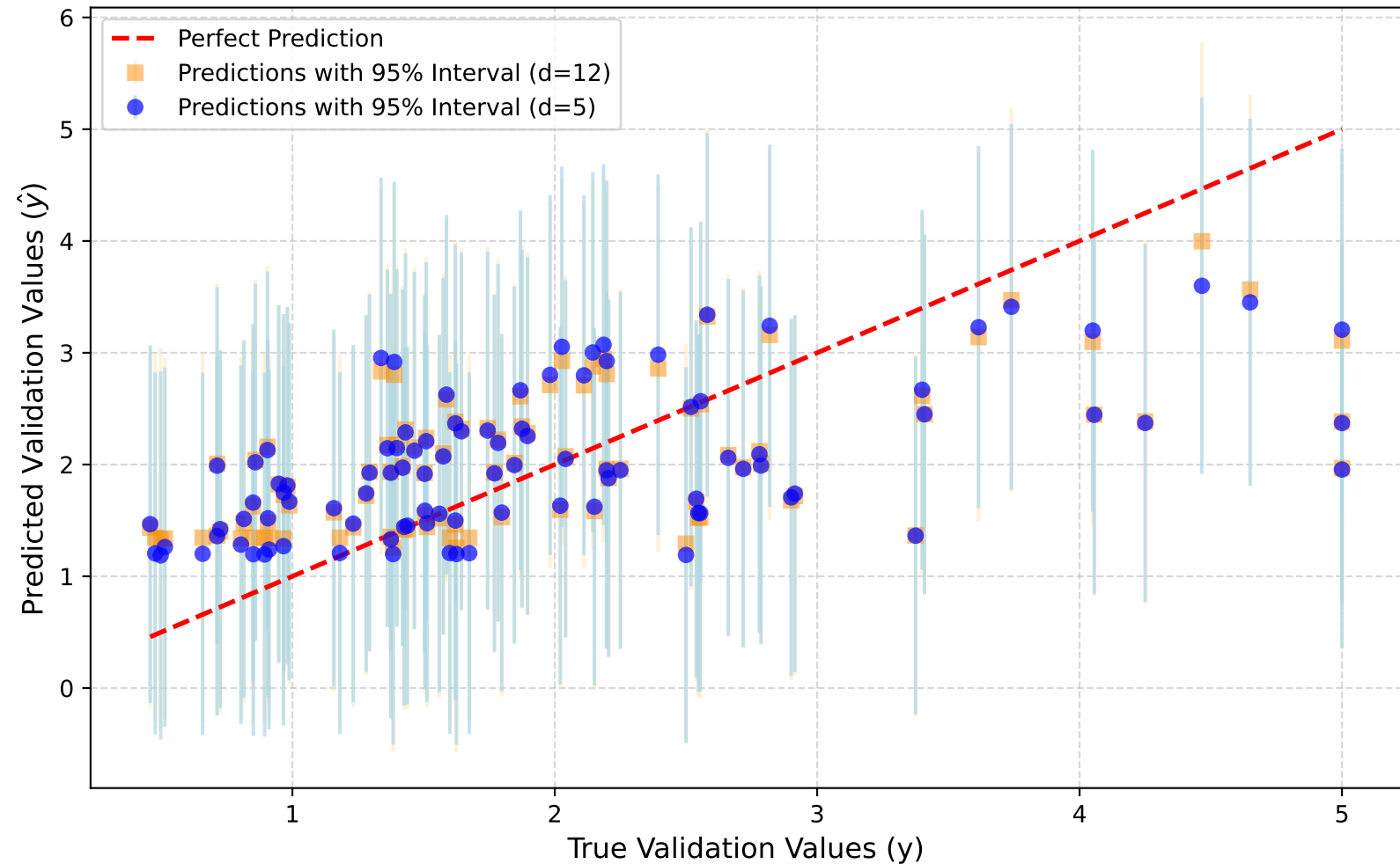
True vs. Predicted Values with 95% Prediction Intervals
