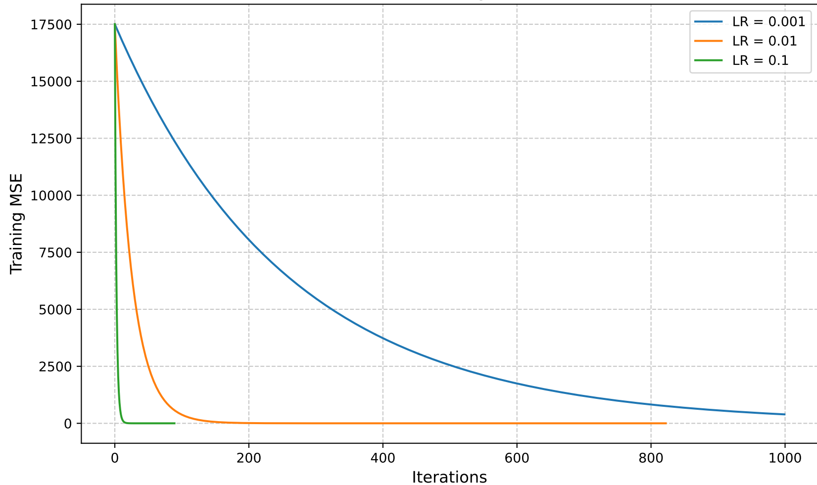
Gradient Descent: Training MSE vs. Iterations
