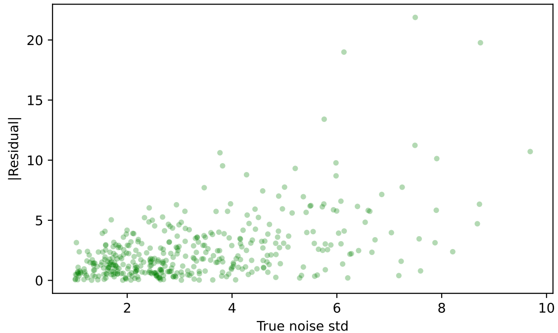
WLS: residuals vs noise level
