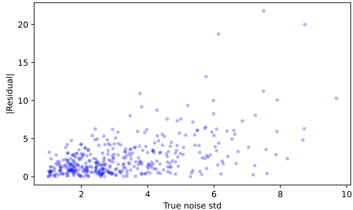
OLS: residuals vs noise level
