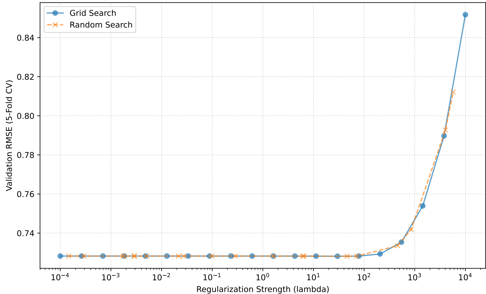
Hyperparameter Search: Grid vs Random (California Housing)
