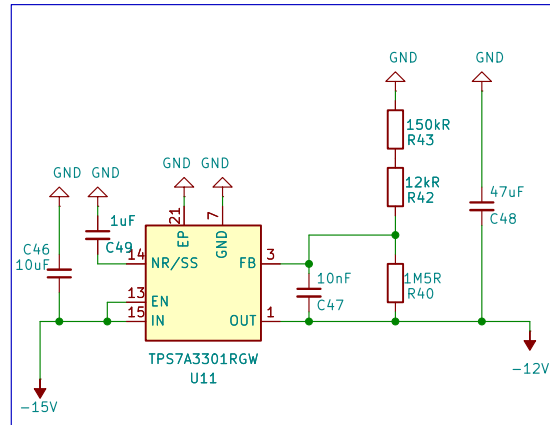
-15V -> -12V
