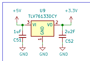
+5V -> +3.3V
