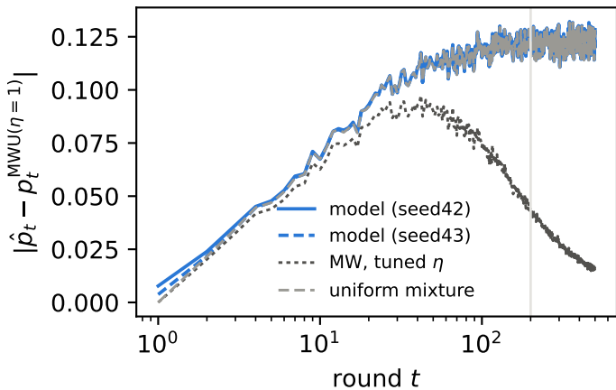
Distance to MWU ( \eta = 1 )
