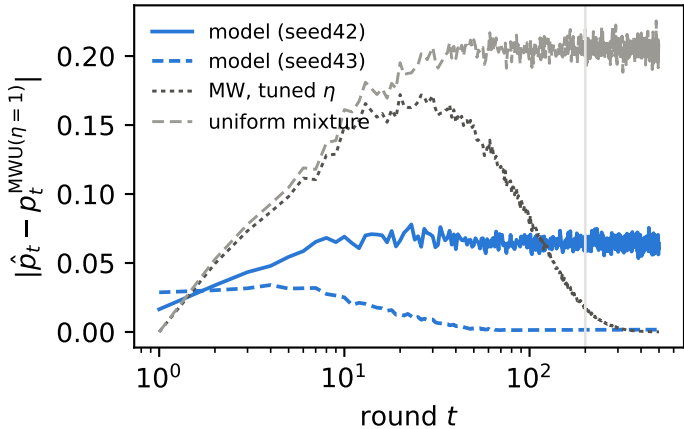
Distance to MWU ( \eta = 1 )
