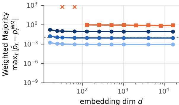
(c) random embeddings
