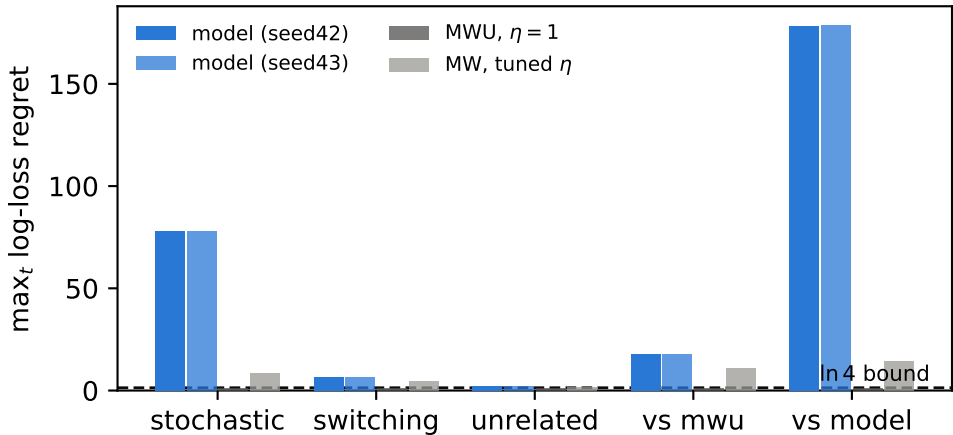
Adversarial sequences (T=500)
